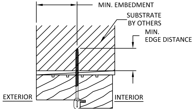
B 12 ANCHOR DETAIL THRU FRAME (HEAD) NOTE: • JAMB HAS SIMILAR DETAIL.
