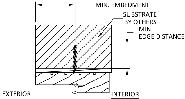
A 12 ANCHOR DETAIL THRU FRAME (HEAD) NOTE: • JAMB HAS SIMILAR DETAIL.
