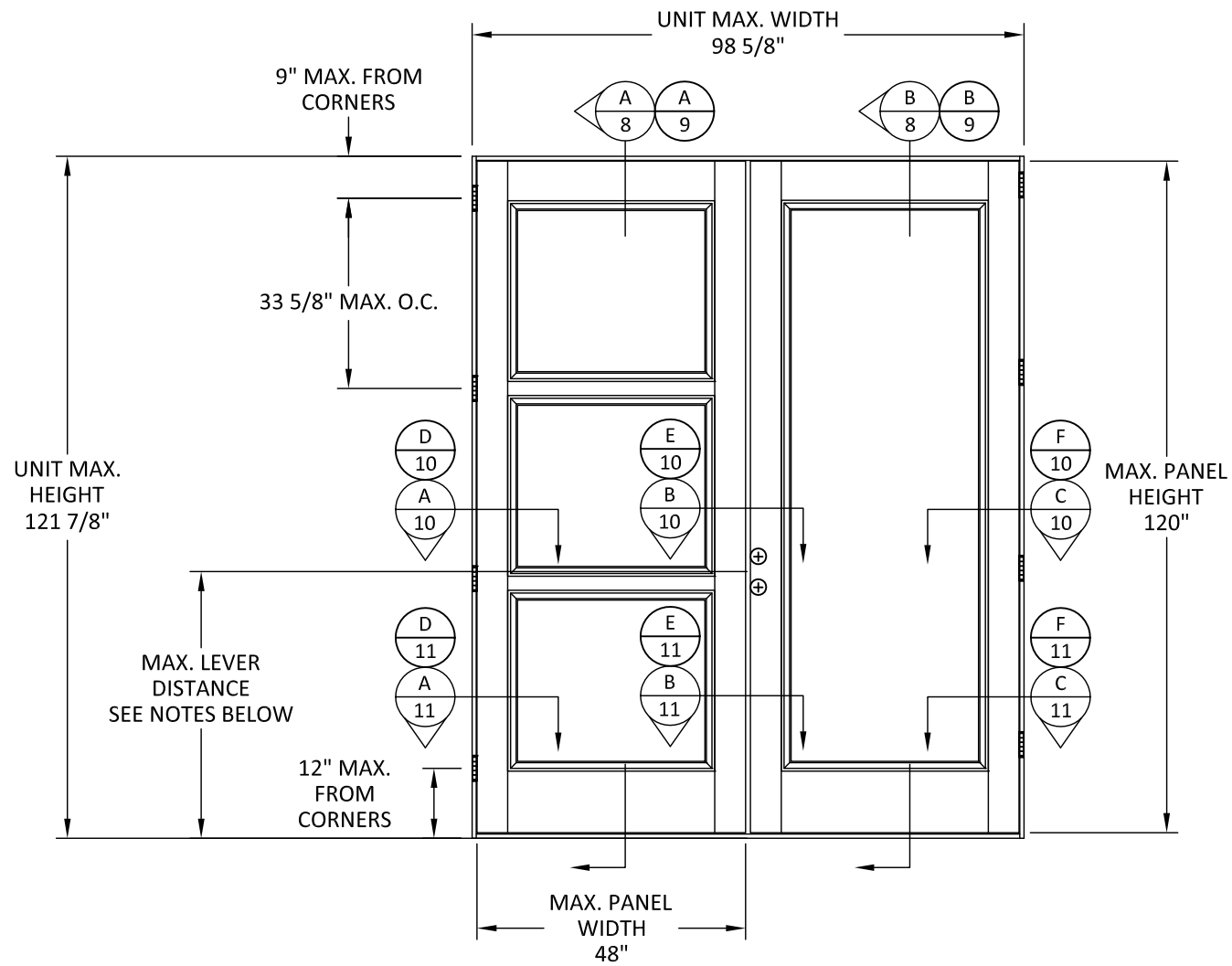
TYPICAL ELEVATION
