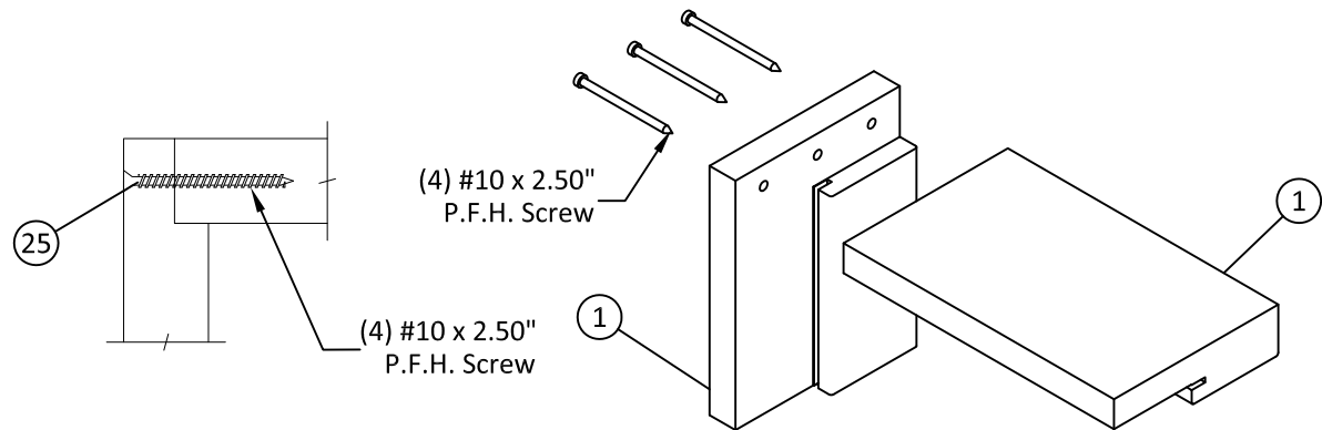
A 17 CORNER SECTION HEAD FRAME ASSEMBLY
