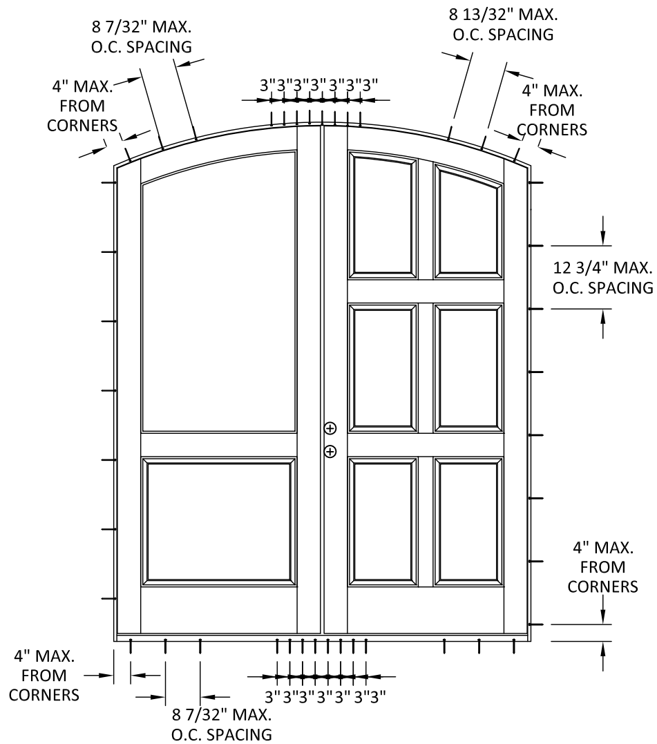
ANCHOR LAYOUT
