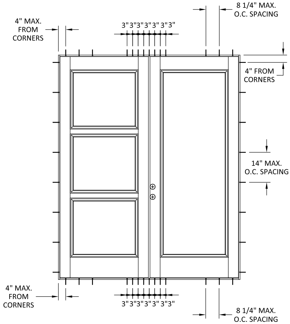
ANCHOR LAYOUT
