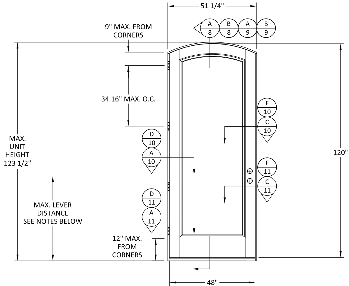
TYPICAL ELEVATION
