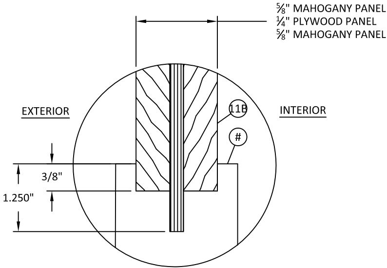
PANEL DETAIL 2 ALL WOOD
