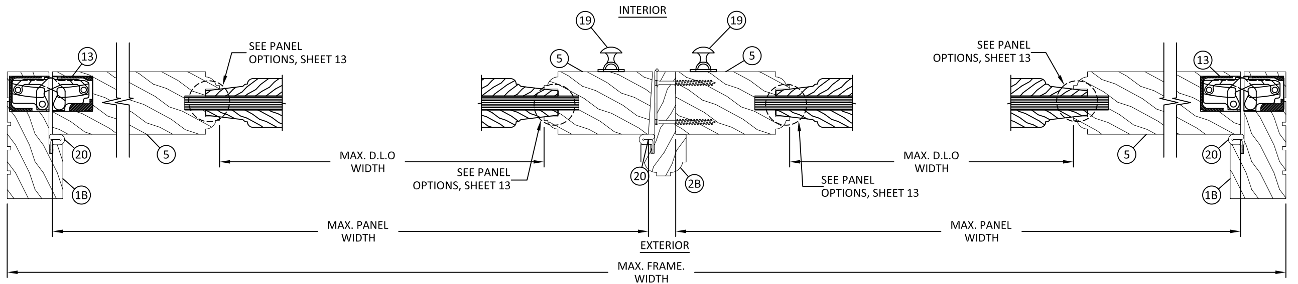
D HORIZONTAL SECTION 11 JAMB INSWING - CONCEALED HINGE
