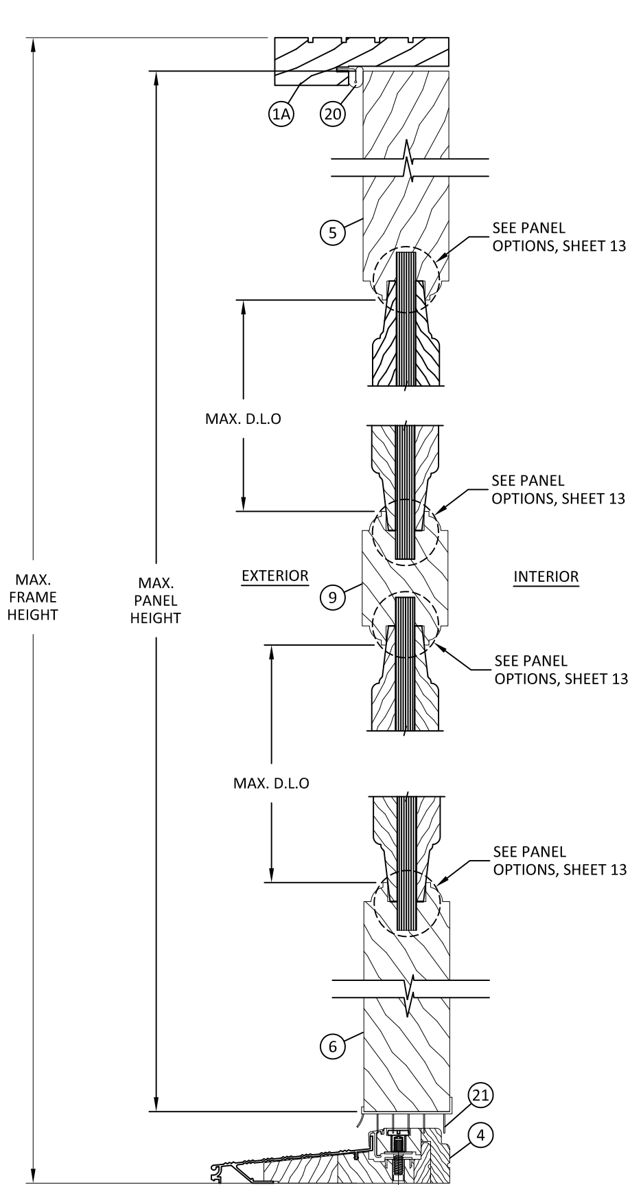
A 9 VERTICAL SECTION INSWING SECTION - BUTT HINGE
