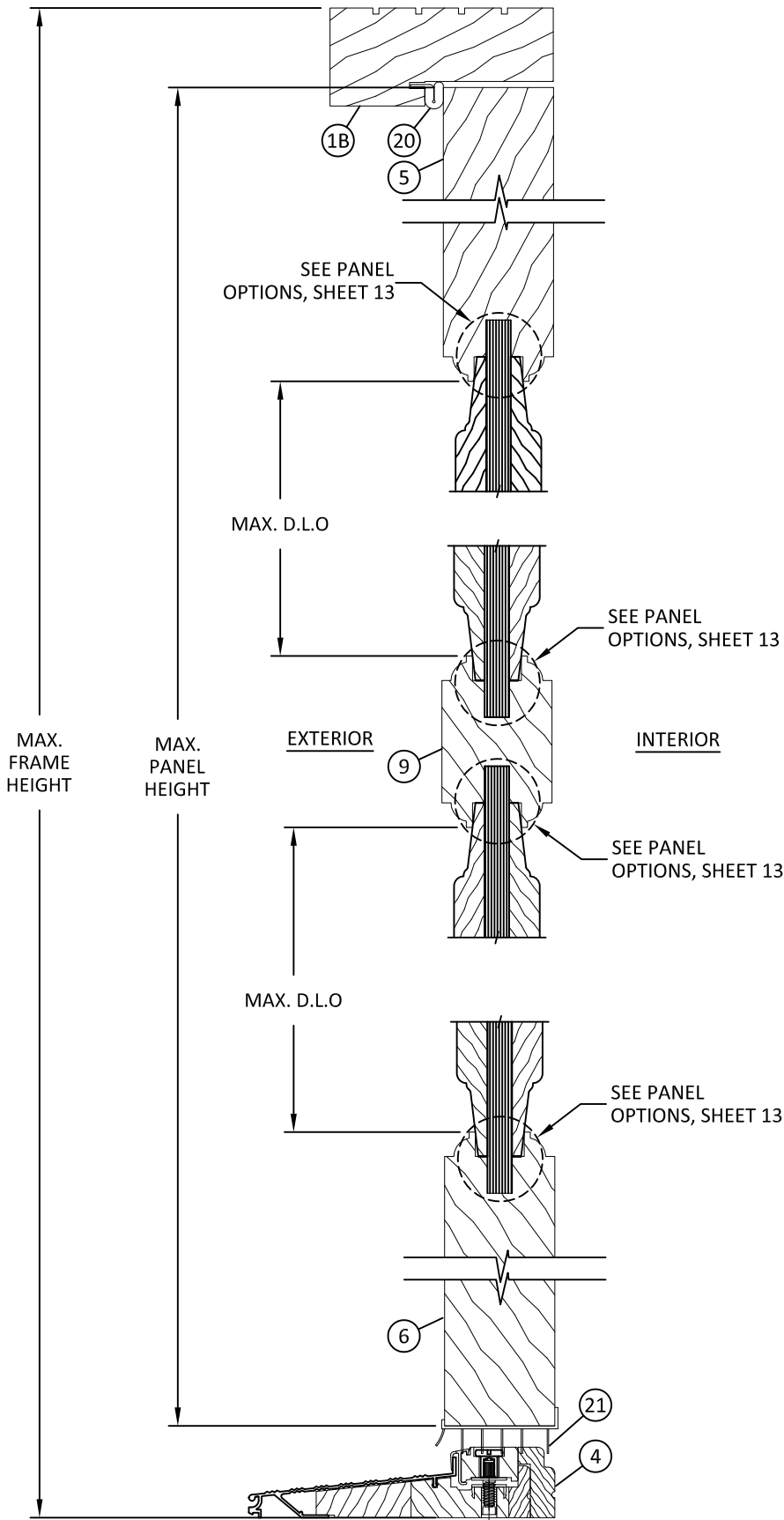
B 9 VERTICAL SECTION INSWING SECTION - CONCEALED HINGE
