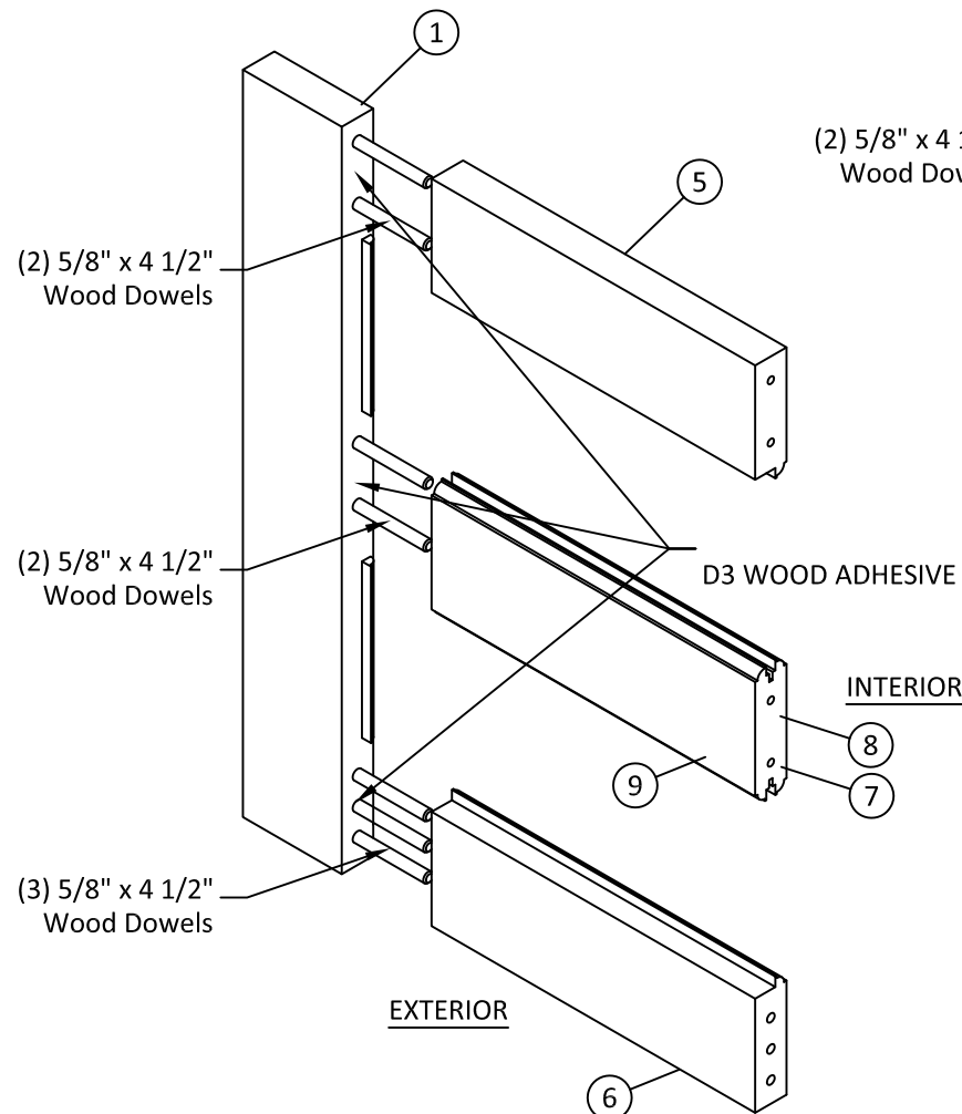
C 17 CORNER SECTION TOP/BOTTOM PANEL ASSEMBLY, TYP.
