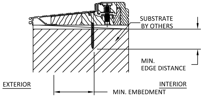
B 12 ANCHOR DETAIL THRU FRAME (HEAD) NOTE: • JAMB HAS SIMILAR DETAIL.
