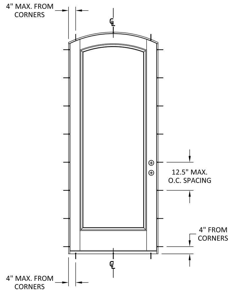
ANCHOR LAYOUT
