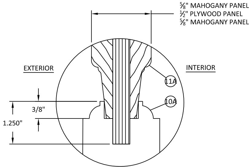
PANEL DETAIL 1 ALL WOOD
