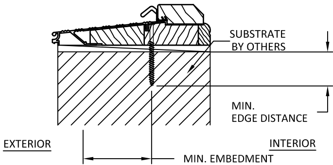
A 12 ANCHOR DETAIL THRU FRAME (HEAD) NOTE: • JAMB HAS SIMILAR DETAIL.
