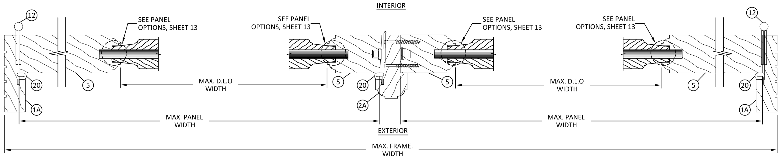
A HORIZONTAL SECTION 11 JAMB INSWING - BUTT HINGE
